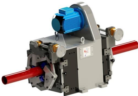
Rotating heads For longitudinal defects detection. For product Ø 1 to 220 mm
