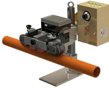
Sectorial magnetizing unit for weld inspection. For product from Ø 5 mm
